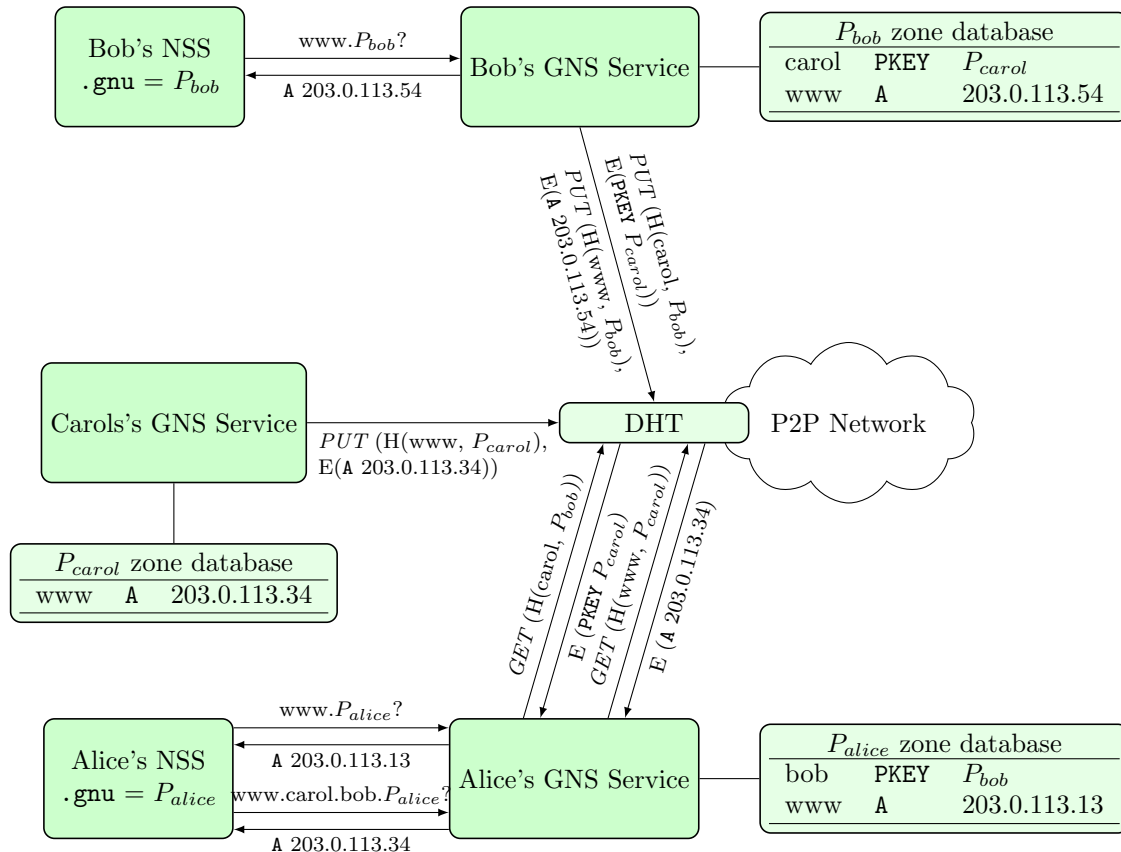
Figure 12: The GNU name system: with GNS, every user maintains their own databases containing record sets under labels organized in zones. A zone is referenced by a public-key pair. Here Alice, Bob and Carol have web servers all reachable under www.gnu . For Alice www.gnu resolves to a different address than for Bob or Carol, as their respective local name service switches (NSS) associate a user-specific public key with .gnu . To allow other users to resolve the names, a user’s public zone information is encrypted and published in a DHT under an obfuscated query key. A user can delegate to another user’s namespace from his local namespace to resolve foreign names. Alice can access Bob’s namespace by delegating control over the name bob to P bob in her namespace using a GNS-specific “PKEY” record. This way Alice can access Carol’s webserver using the name www.carol.bob.gnu .
