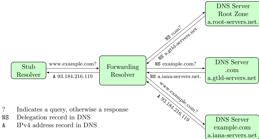
Figure 8: With query minimization, resolving the name www.example.com no longer exposes the full name and query type to the root zone and the .com authority. Naturally, this scheme still leaks quite a bit of sensitive information to the TLD’s DNS server. Furthermore, the effect is even weaker in practice, as root zone is already often not contacted as information about TLD name servers is typically cached at forwarding resolvers.
