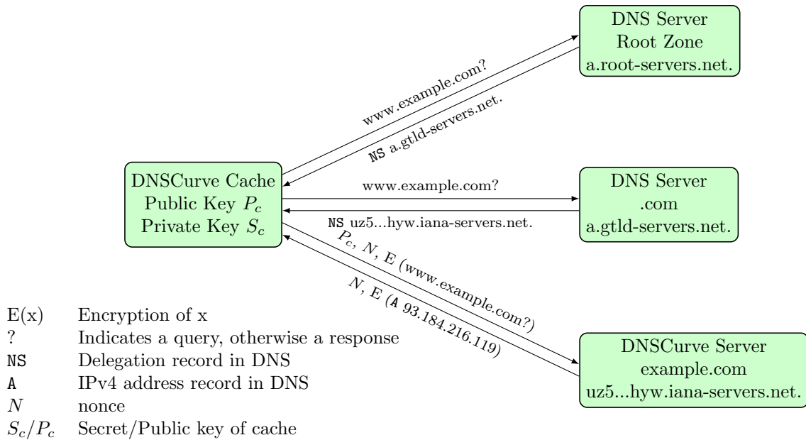
Figure 9: Resolving the name www.example.com with DNSCurve. With DNSCurve, the resolving cache and the DNSCurve server exchange a shared secret to encrypt their communication. The DNSCurve server’s public key is encoded in the name of the name server itself using Base32. When a DNSCurve cache resolves a name and finds the name server to support DNSCurve, the cache creates a shared secret based on the server’s public key, the cache’s private key, and a one-time nonce. The cache sends its public key, the nonce and the query encrypted with the shared secret. The server will respond with the result of the query encrypted with the shared secret. The first two lookups to the root zone and the “.com” TLD do not use DNSCurve in the illustration as those currently do not support DNSCurve.
