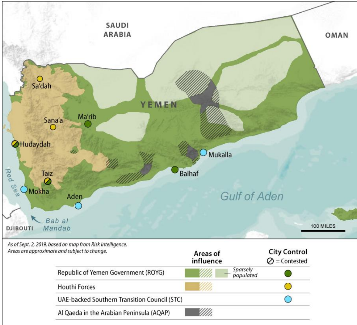
Figure 1. Lines of Control in Yemen As of September 2019
